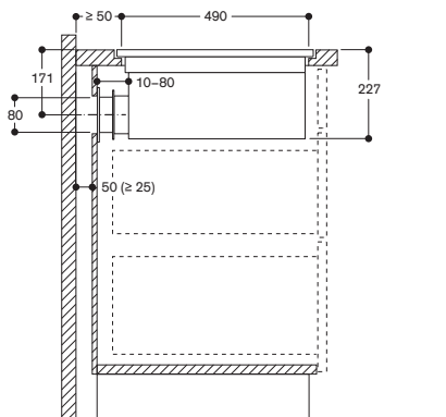
Not recommended for non-thermally insulated outer wall or floor (U ≥ 0.5 W/m 2 K)
