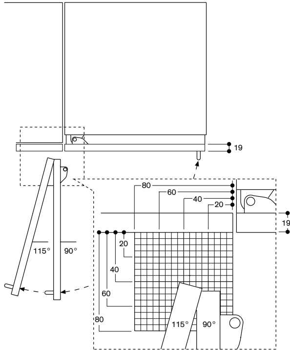
Deuropeningshoek
