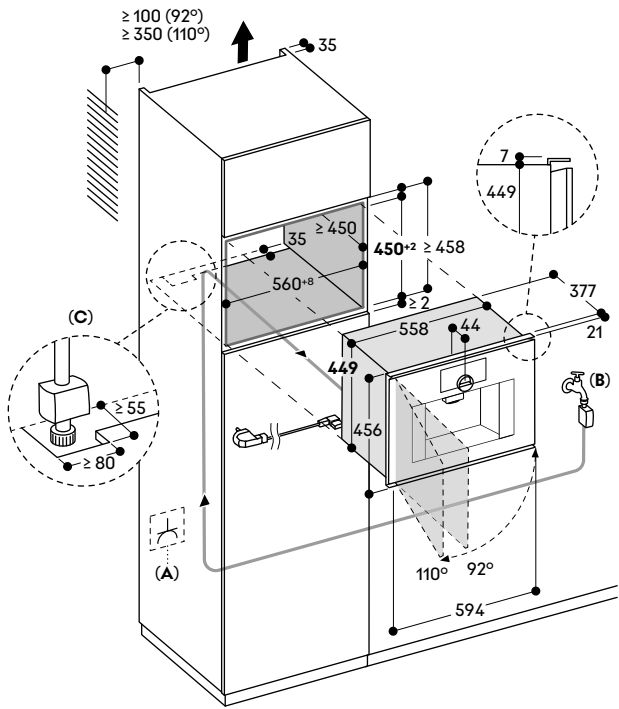
A: Accessible electrical connection B: Accessible water connection C: Additional cut-out to pass Aquastop
