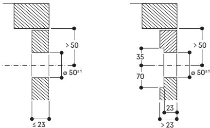
Installation of the control ring Surface mounting
