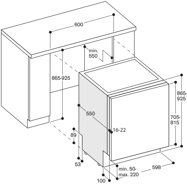
86.5 cm high dishwasher with flexible hinge
