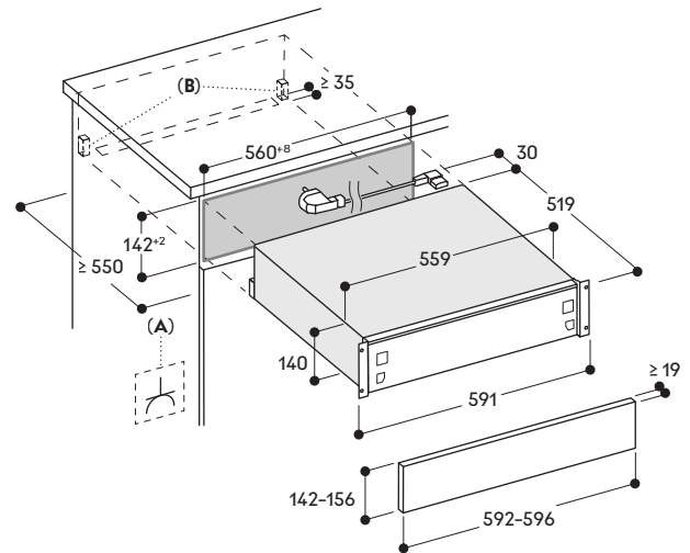
A: Accessible electrical connection B: Anti tilting
