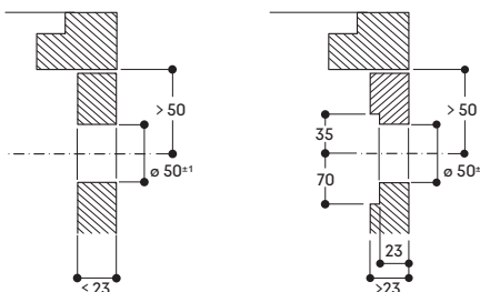
Installation of the control ring Flush installation
