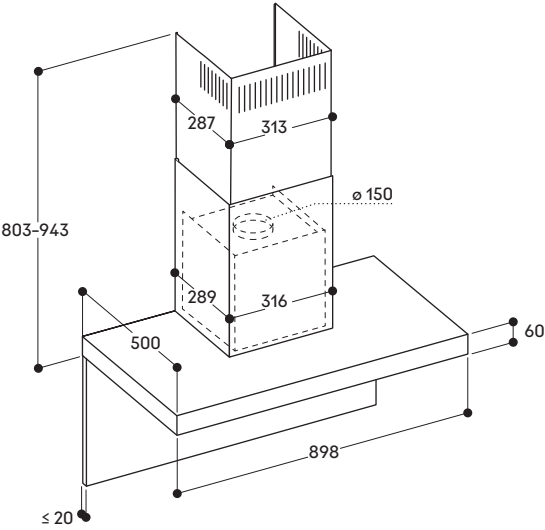
AW 290 with AA 290 800
