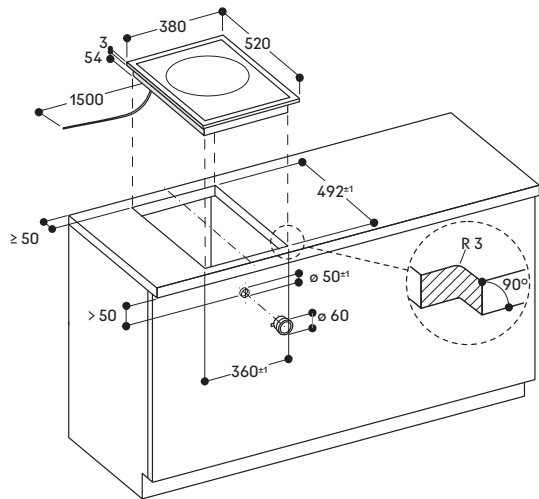
Installation of the cooktop; surface mounting
