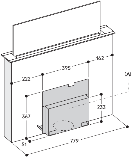
AL 200 181 with AA 200 910
