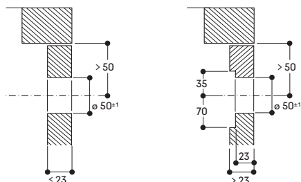
Installation of the control ring Surface mounting
