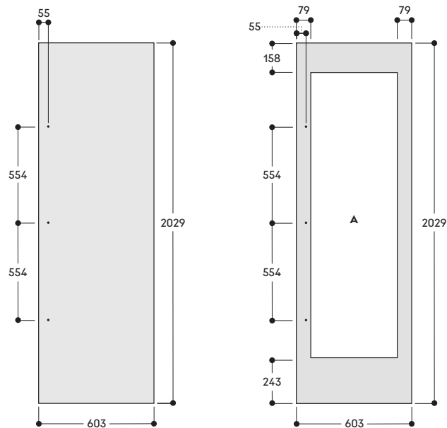
Niche width 610 mm
