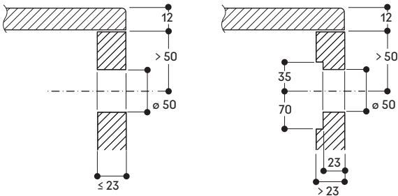
Installation of the control ring
