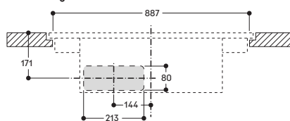
Front view - furniture cut-out for unducted recirculation; flush mounting
