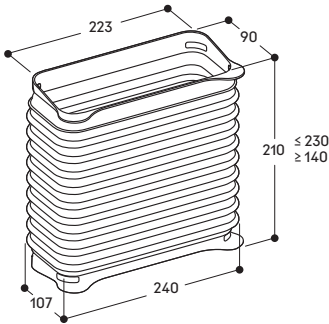
AD 410 040 : Flexibel connecting piece, DN 150 flat
