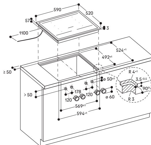
Installation of the cooktop; flush mounting
