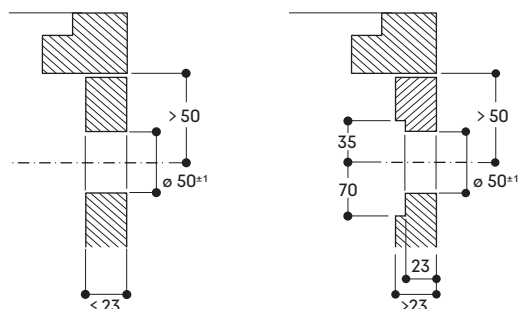
Installation of the control ring Flush installation
