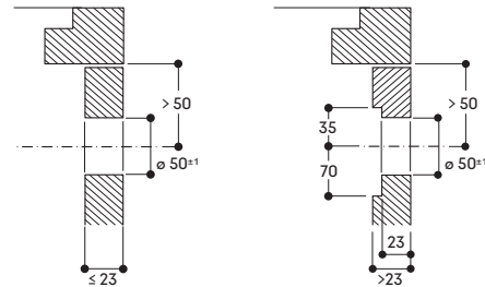
Installation of the control ring Flush installation
