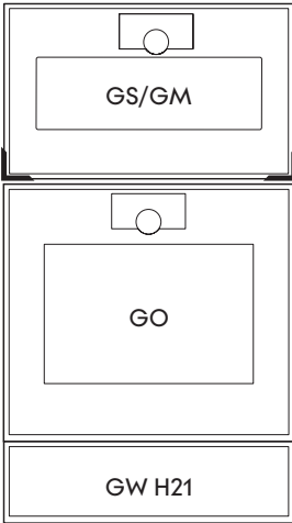
Combination EV3_21_H45 (For dimensions, see page 18)
