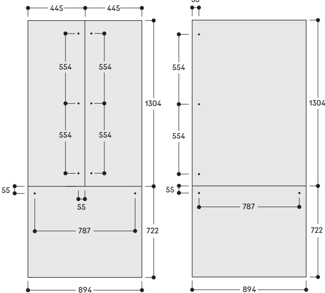
Niche width 900 mm
