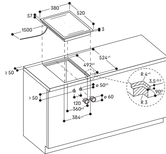
Installation of the cooktop; flush mounting
