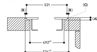
Cross-section
