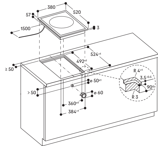
Installation of the cooktop; flush mounting
