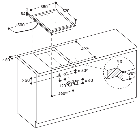
Installation of the cooktop; surface mounting
