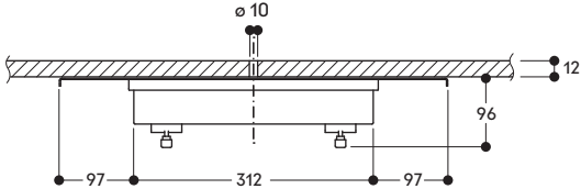
Cross section
