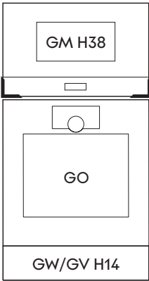
Combination MV6_14_H38 (For dimensions, see page 63)
