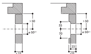
Installation of the control ring Flush installation
