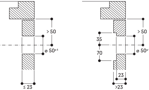
Installation of the control ring Flush installation
