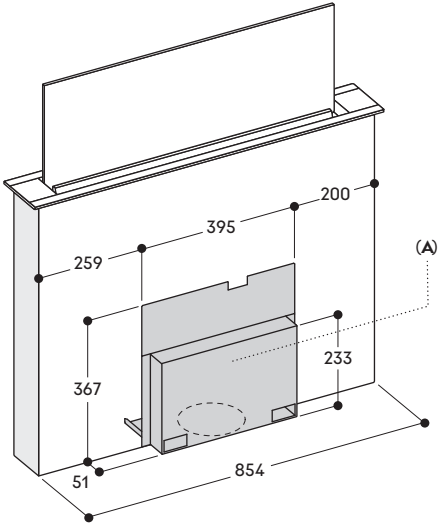
AL 200 191 with AA 200 910
