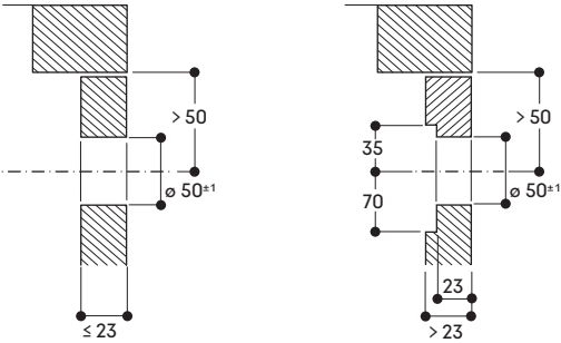
Installation of the control ring Surface mounting
