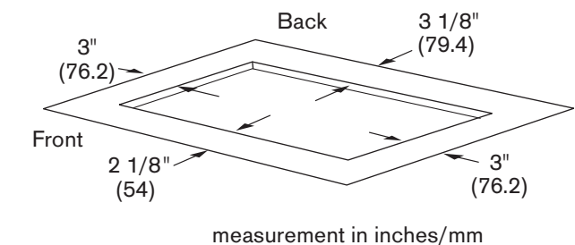
Figure 3: Cutout Dimensions
