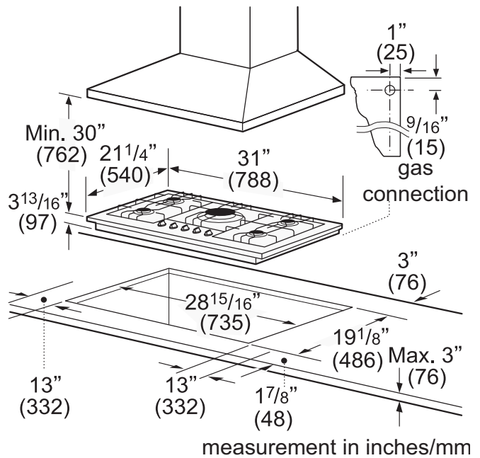
Figure 2: Cutout Dimensions
