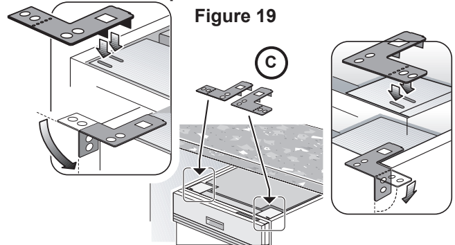
Top and Side Mount
