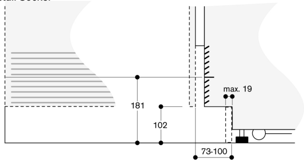
Detail Sockel
