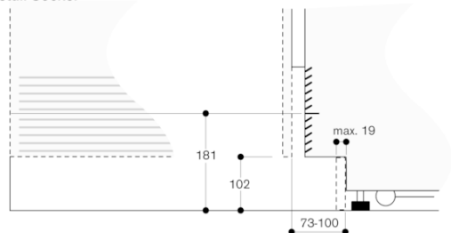
Detail Sockel
