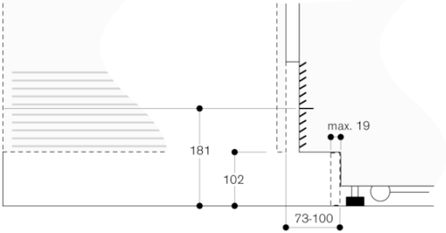
Detail Sockel
