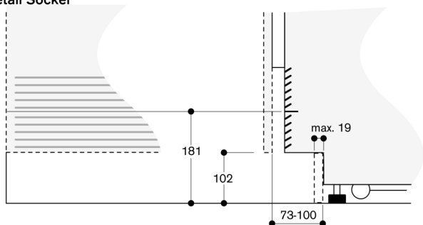
Detail Sockel
