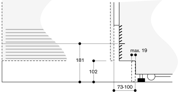
Detail Sockel
