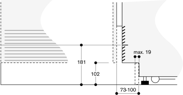
Detail Sockel
