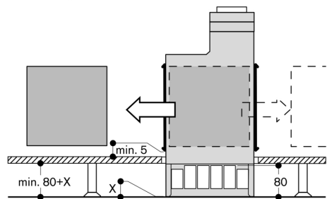
Filter exchange
