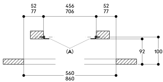
A: Mounting brackets Measurements in mm
