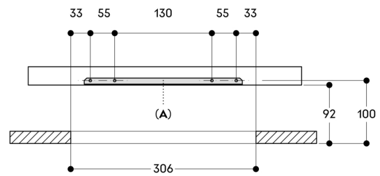
A: Mounting brackets Measurements in mm
