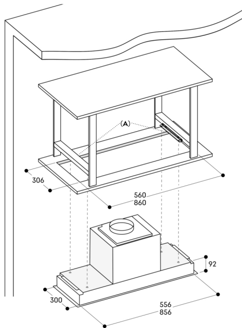
A: Mounting brackets Measurements in mm
