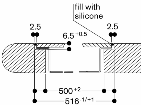
Cross-section
