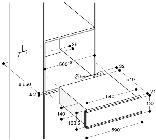
Socket measurements in mm
