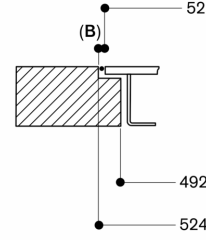
Cross-section
