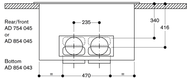
AL 400 connection positions DN 150
