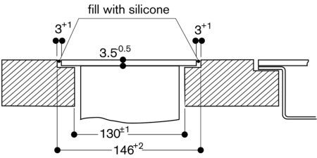
Cross-section
