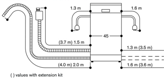
Connection dimensions for a 45 cm wide dishwasher
