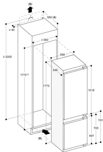
A: 560 mm recommended, min. 550 mm B: min. 200 \text{cm}^2 A: Socket measurements in mm
