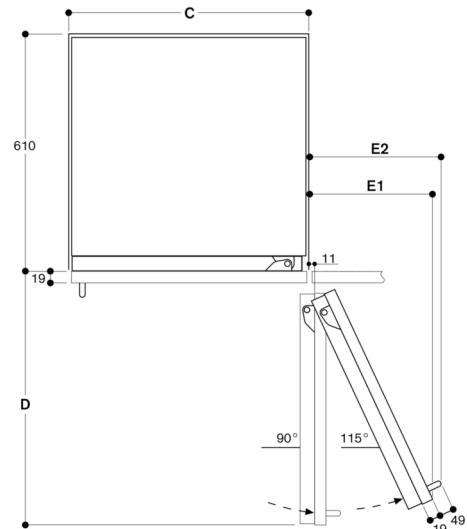
Wall clearance RB 472/RC/RF/RW
