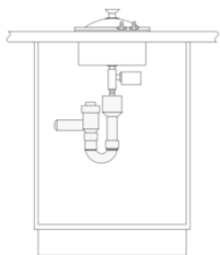
Drainage connection present in the bottom cupboard: Fixed connection with free fall section as per DIN 1986 Part 1. A non-return valve must be installed. Recommendation: Install a non-return valve. Recommendation: AG 050 000 Drain installation set.
