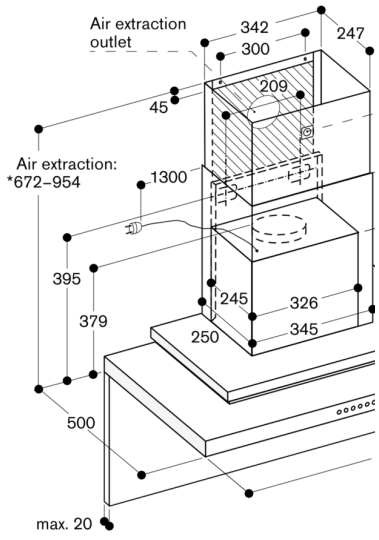
AW 230 with AA 200 812
