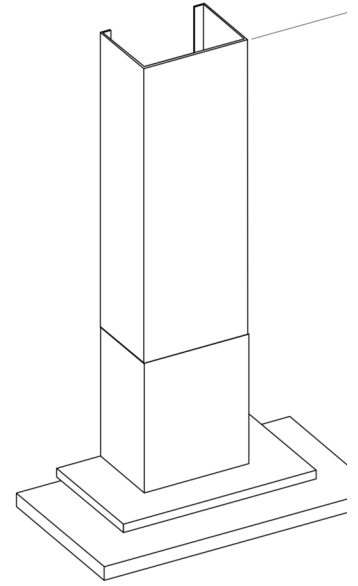
AW 230 with AD 200 322
