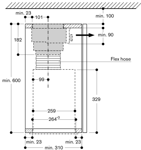
Cross-section top cabinet with AC 200 and AA 211 812
