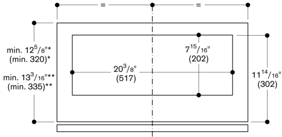
Top view of top cabinet with AA 211 812
