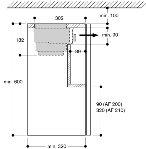
Cross-section top cabinet with AA 211 812
