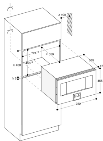
Socket measurements in inches (mm)
