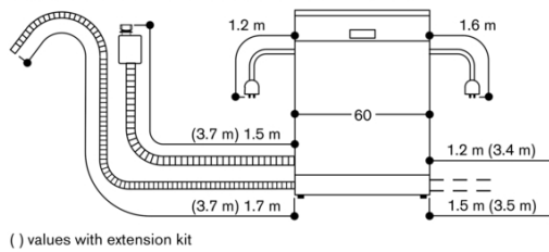
Connection dimensions for a 60 cm wide dishwasher
