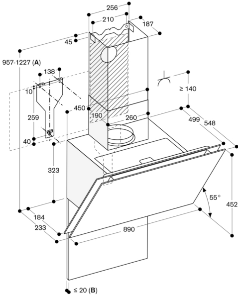
Air extraction
