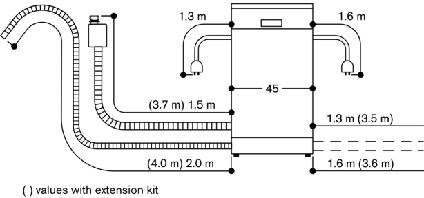
Connection dimensions for a 45 cm wide dishwasher
