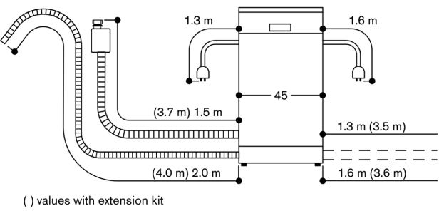
Connection dimensions for a 45 cm wide dishwasher
