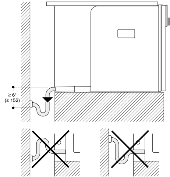
Raccordement d'évacuation
