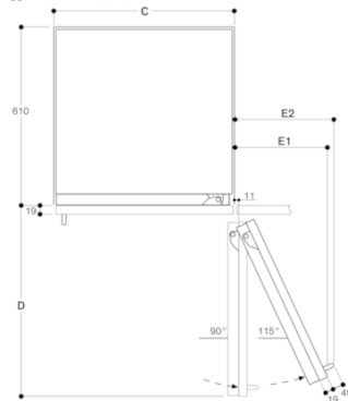
Veggavstand RB 472/RC/RF/RW
