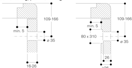
Vredmontering, planmontering
