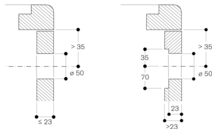
Vredmontering, planmontering
