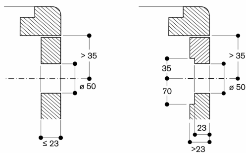
Vredmontering, planmontering
