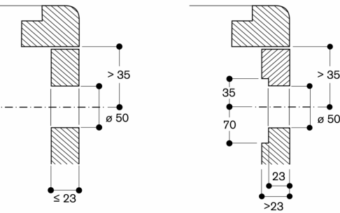
Vredmontering, planmontering
