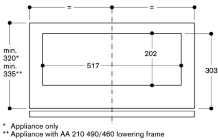
View of upper cabinet from above with AA 211 812
