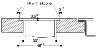
Cross-section
