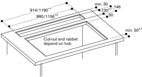
AL 400 installed flush
