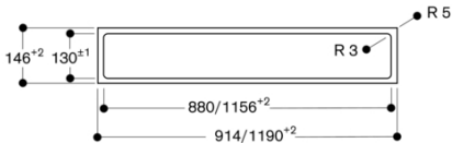
AL 400 cut-out flush-mounted
