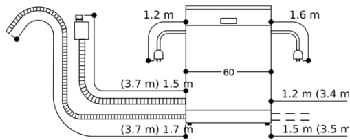
60 cm寬的洗碗機的連接尺寸
